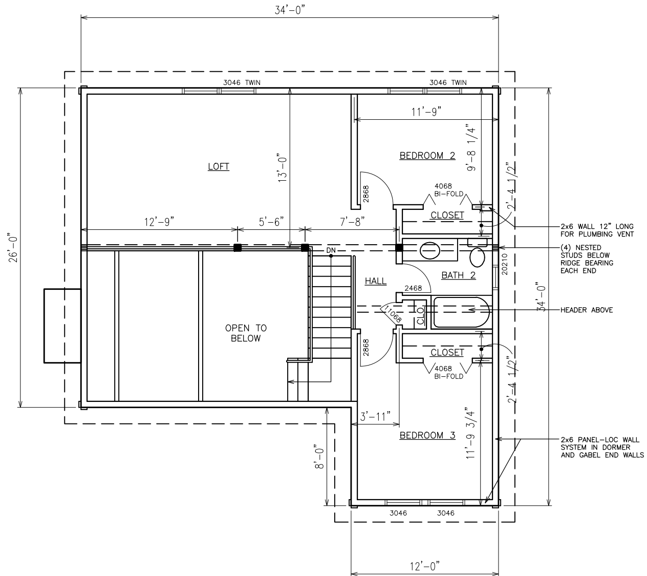
STONEY CREEK - SECOND FLOOR PLAN 3 BEDROOMS, 2 BATHS, 1,960 SQUARE FEET
