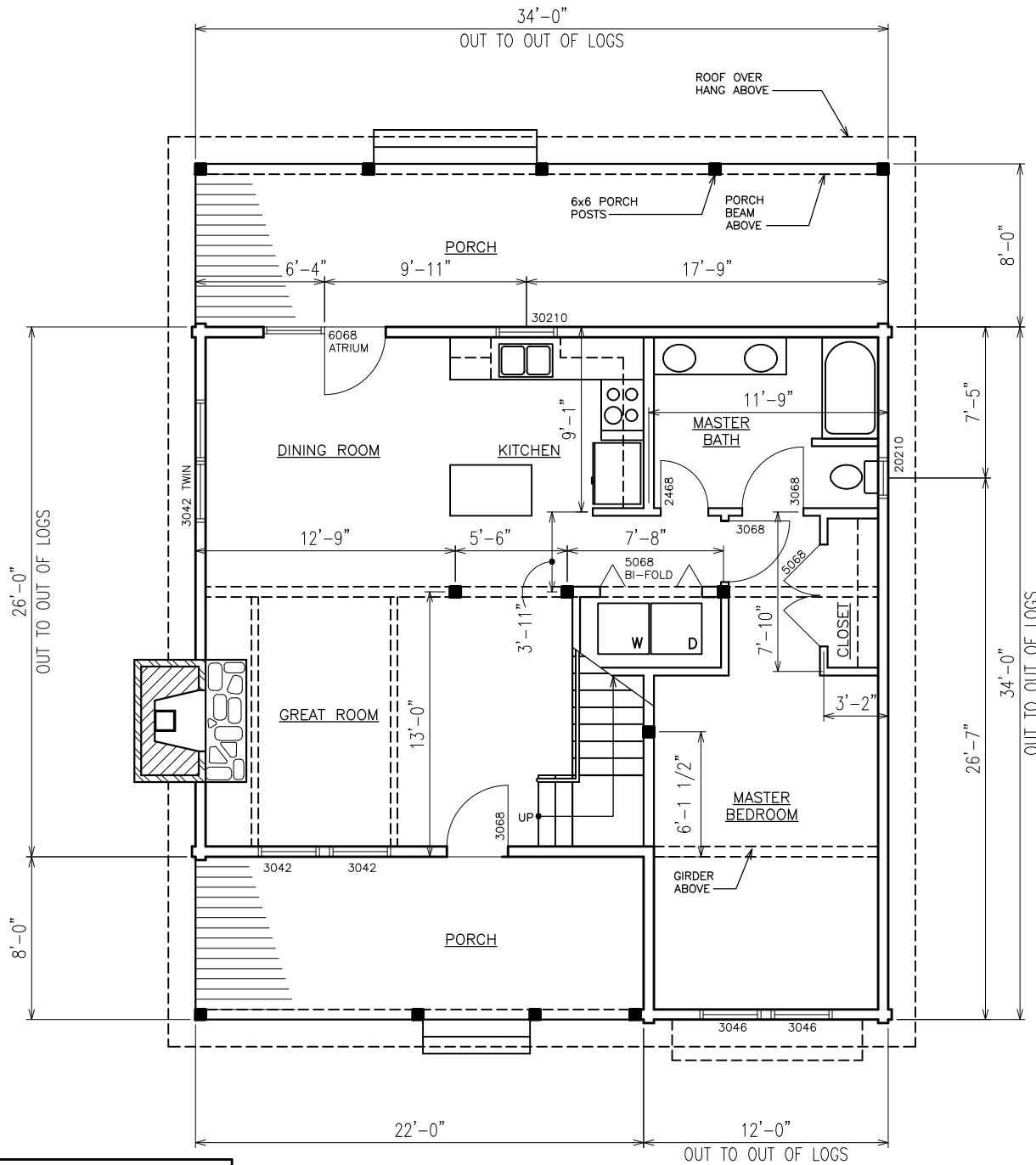
STONEY CREEK - FIRST FLOOR PLAN 3 BEDROOMS, 2 BATHS, 1,960 SQUARE FEET
