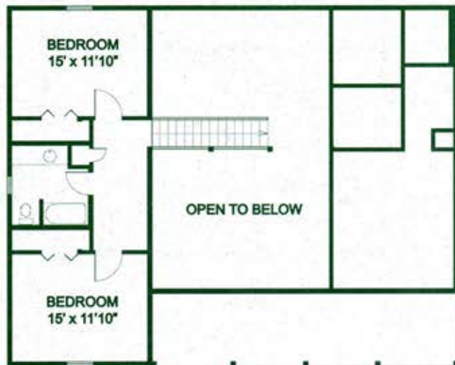
SECOND FLOOR
