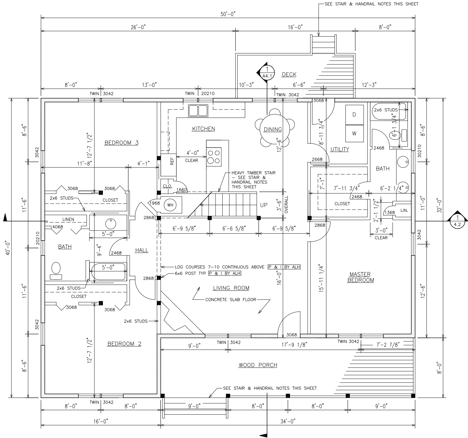
A1 FIRST FLOOR PLAN 1728 S.F. 1/8" = 1'-0"
