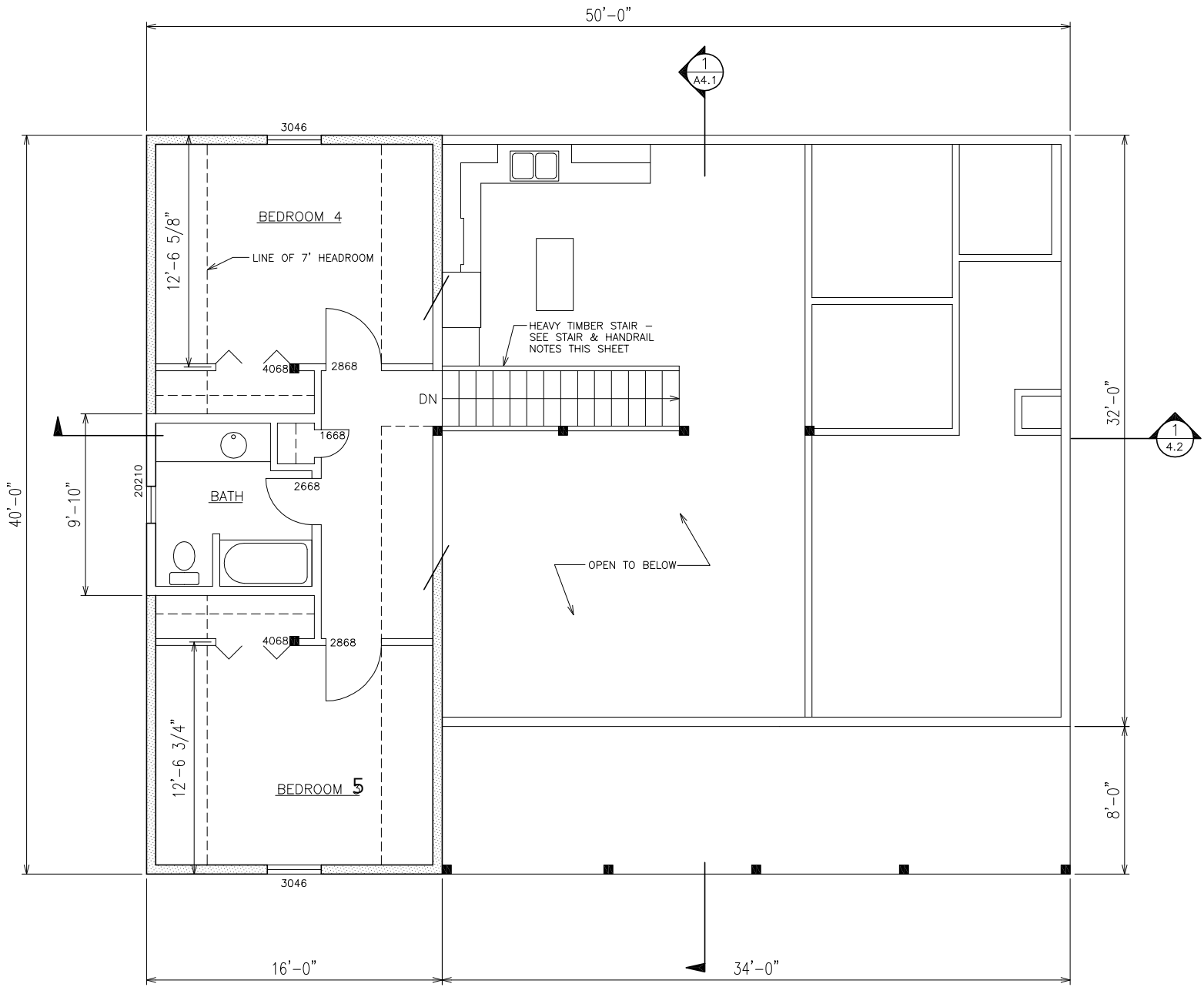
A1 SECOND FLOOR PLAN 1/8" = 1'-0" 640 S.F.
