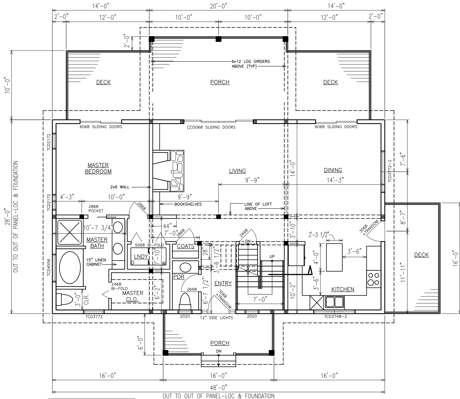
DIVIDE MOUNTAIN - FIRST FLOOR PLAN 3 BEDROOMS, 4 BATHS, 2,611 SQUARE FEET
