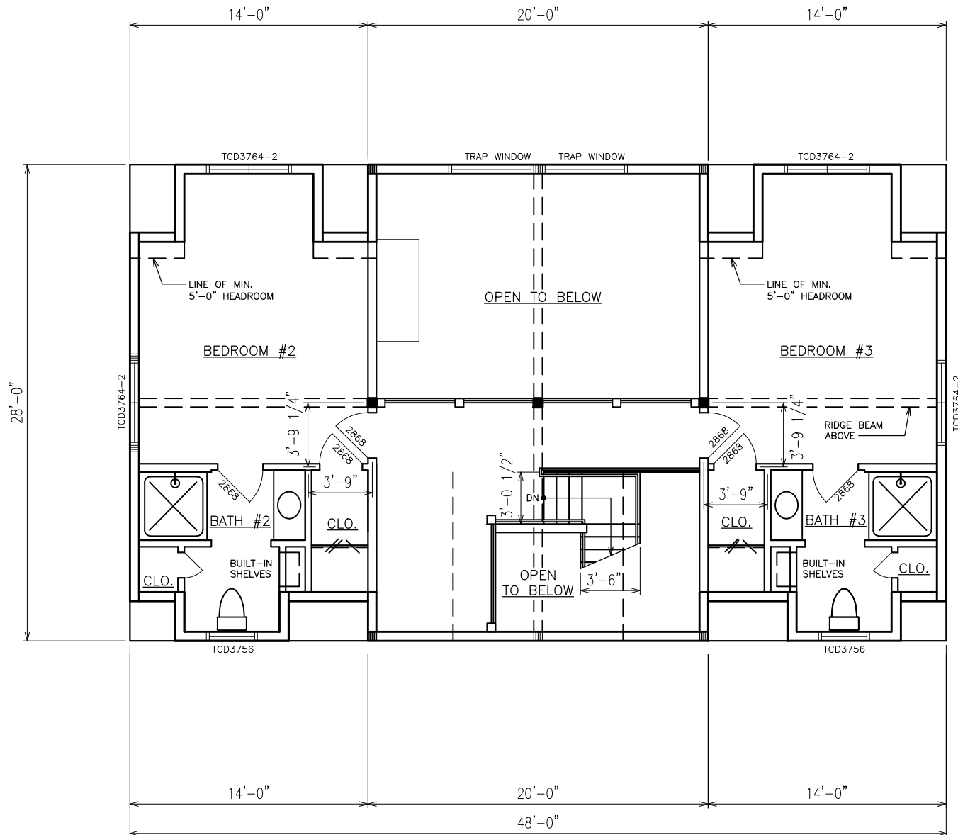
DIVIDE MOUNTAIN - SECOND FLOOR PLAN 3 BEDROOMS, 4 BATHS, 2,611 SQUARE FEET
