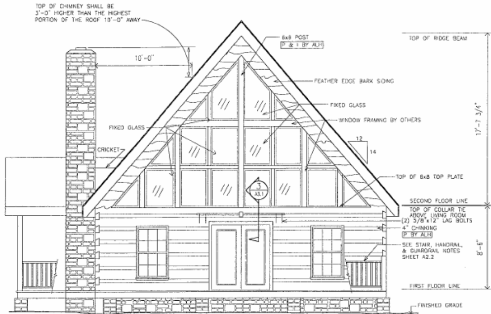
1 FRONT ELEVATION 1/8" = 1'-0"
