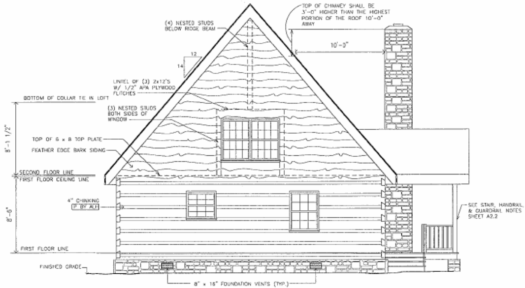
2 REAR ELEVATION 1/8" = 1'-0"
