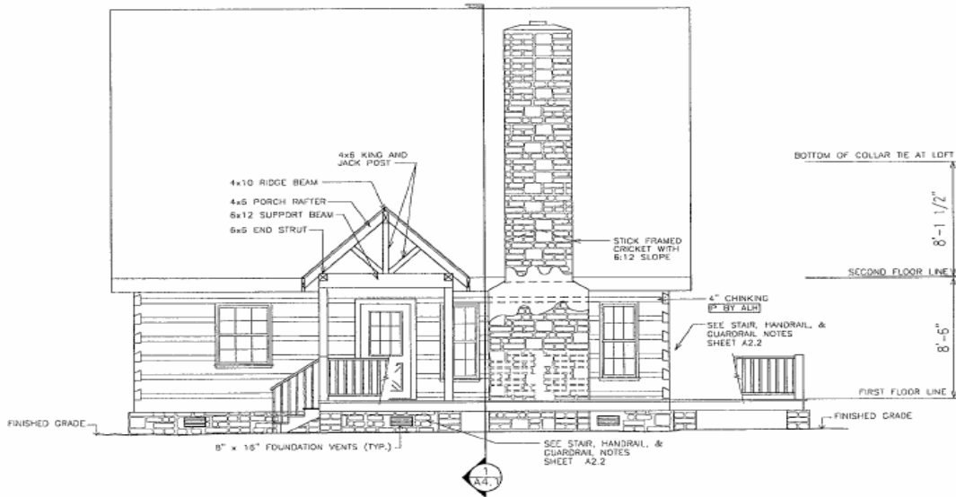
2 LEFT ELEVATION 1/8" = 1'-0"
