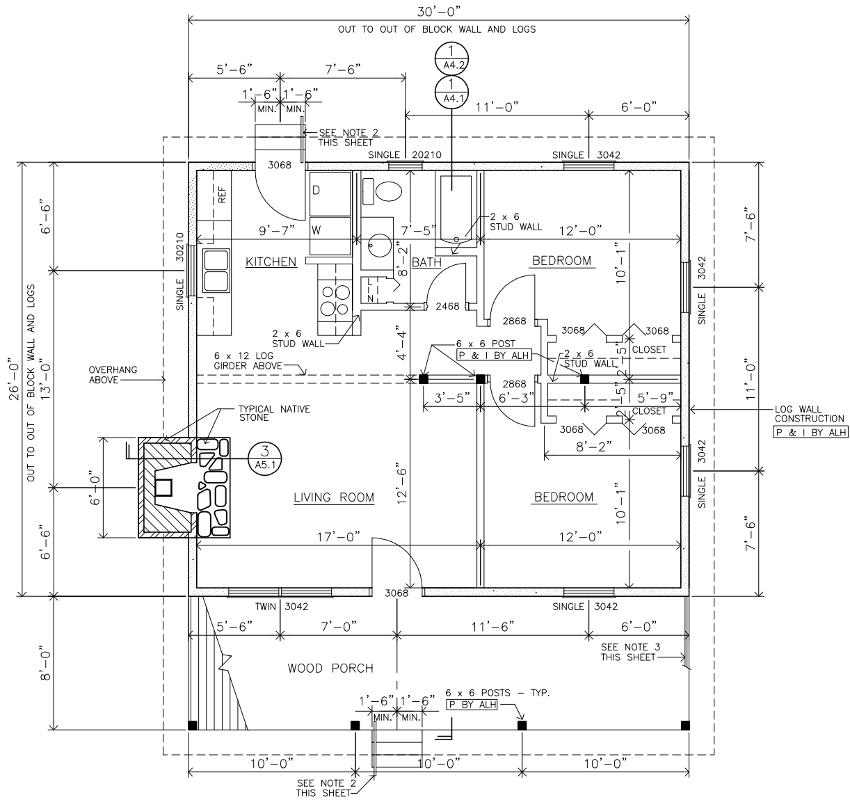
1 FIRST FLOOR PLAN HIWASSEE I A2.2 SCALE: 1/8" = 1'-0"
