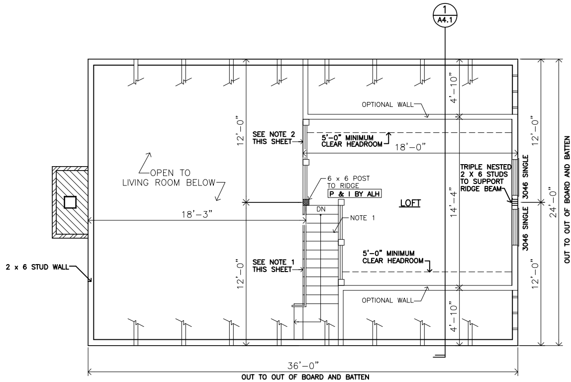
1 A2.4 SECOND FLOOR PLAN SCALE: 1/8" = 1'-0"
