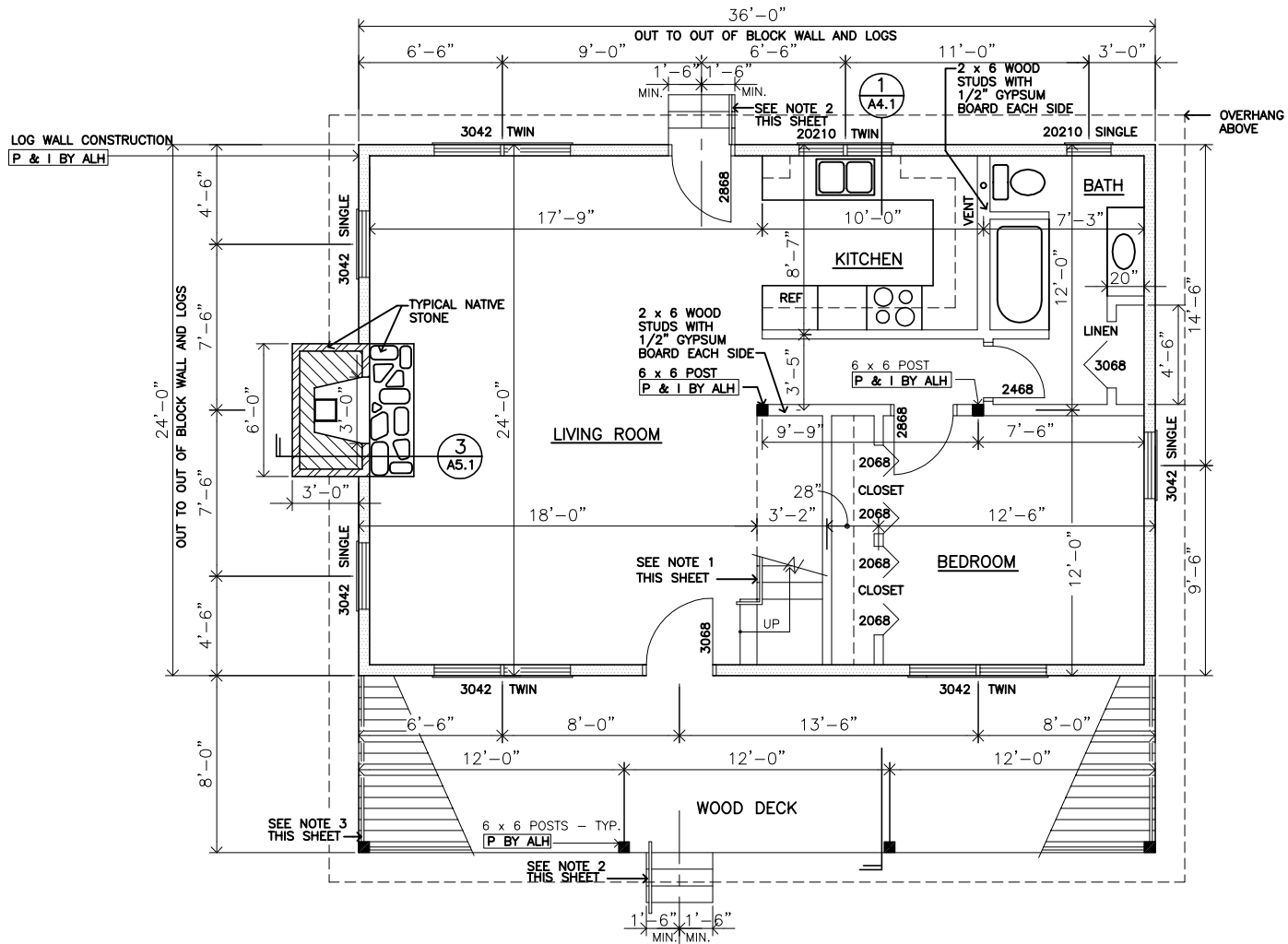
1 FIRST FLOOR PLAN LONESOME PINE II A2.2 SCALE: 1/8" = 1'-0"
