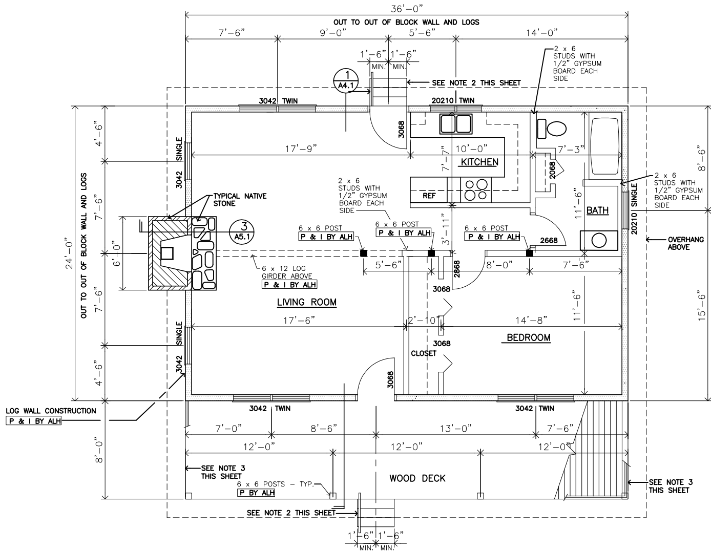
1 A2.2 FIRST FLOOR PLAN LONESOME PINE SCALE: 1/8" = 1'-0"
