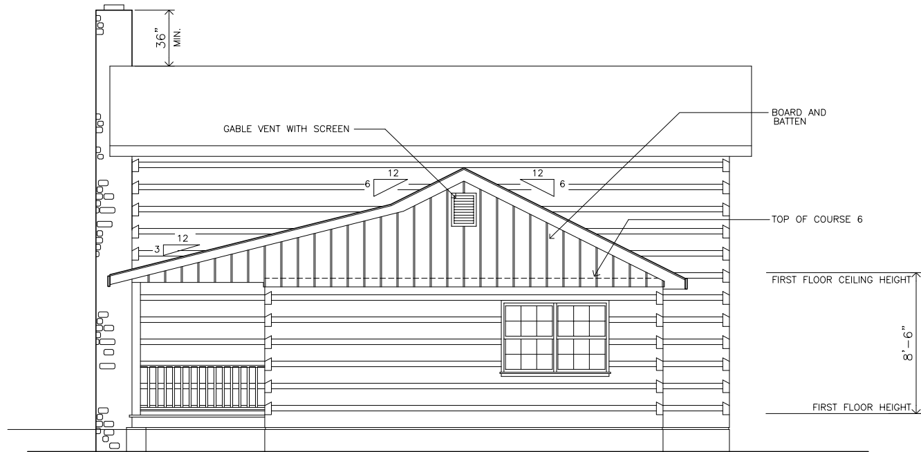
1 A3.2 FRONT ELEVATION SCALE: 1/8" = 1'-0" SANTA FE TRAIL
