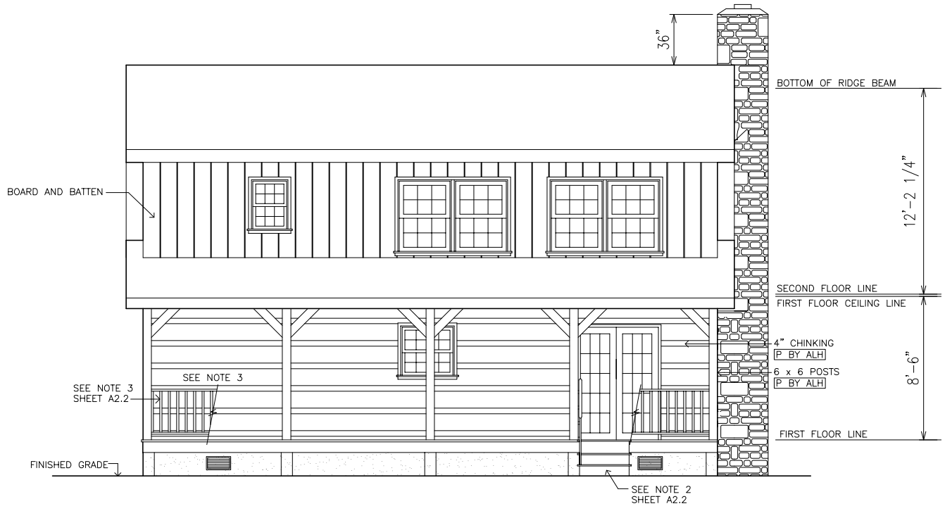
1 A3.2 REAR ELEVATION STONE MOUNTAIN SCALE: 1/8" = 1'-0"
