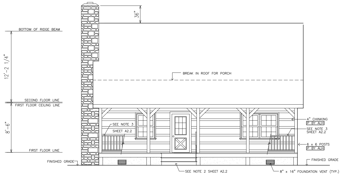
1 A3.1 FRONT ELEVATION STONE MOUNTAIN SCALE: 1/8" = 1'-0"
