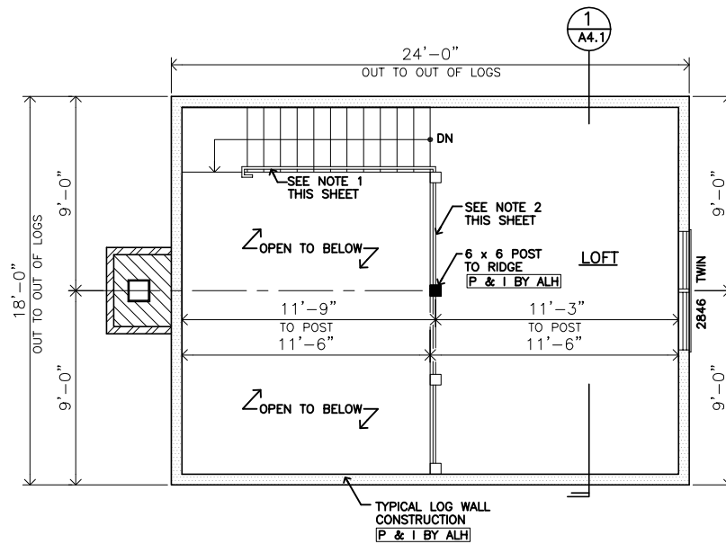
1 SECOND FLOOR PLAN A2.4 SCALE: 1/8" = 1'-0"
