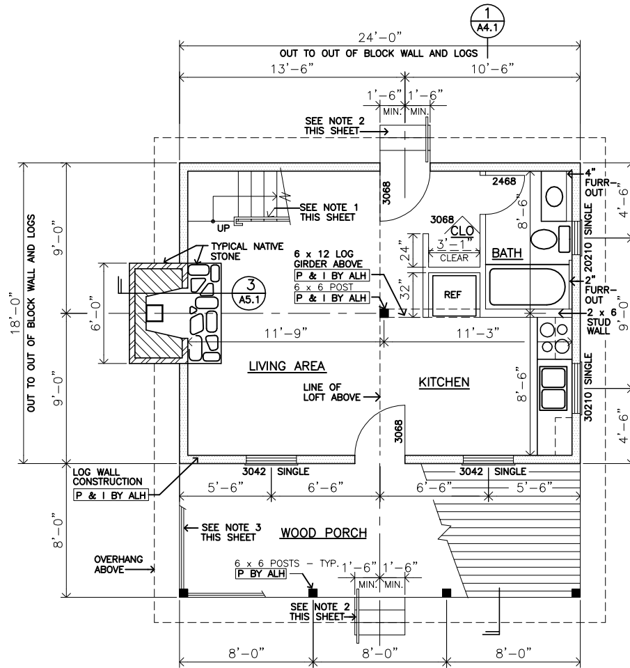
1 FIRST FLOOR PLAN — YUKON TRAIL I A2.2 SCALE: 1/8" = 1'-0"
