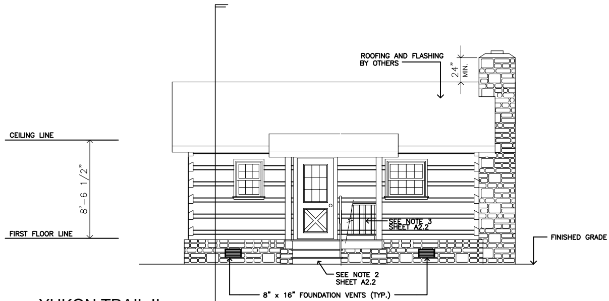
YUKON TRAIL II REAR ELEVATION SCALE: 1/8" = 1'-0"
