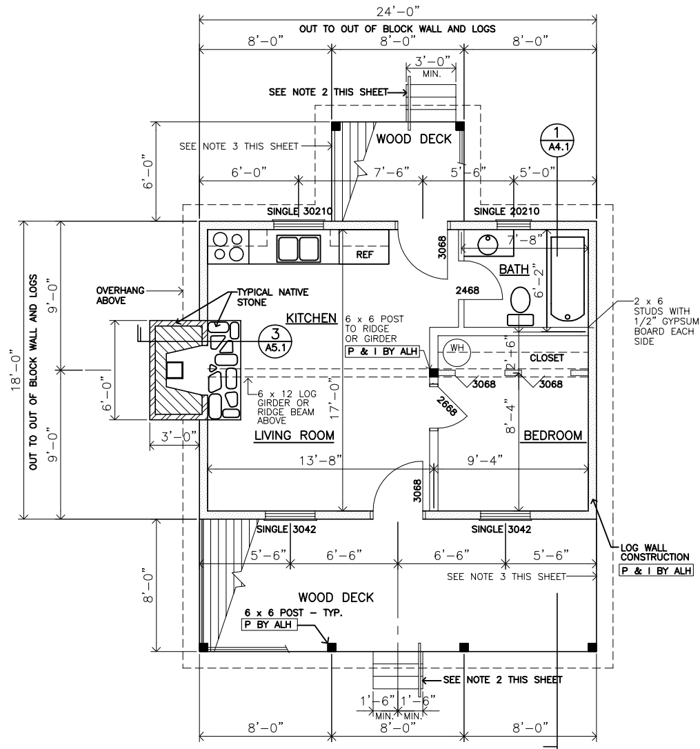
YUKON TRAIL II (1) FIRST FLOOR PLAN (A2.2) SCALE: 1/8" = 1'-0"
